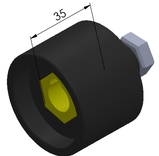
Conector chasis hembra 35-50 ST 13mm Carcasa 49mm
